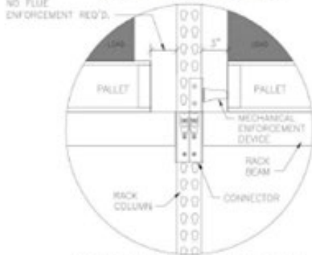
DETAIL 1 MECHANICAL ENFORCEMENT DEVICE AT RACK COLUMN (NET 3" TRANSVERSE FLUE)
