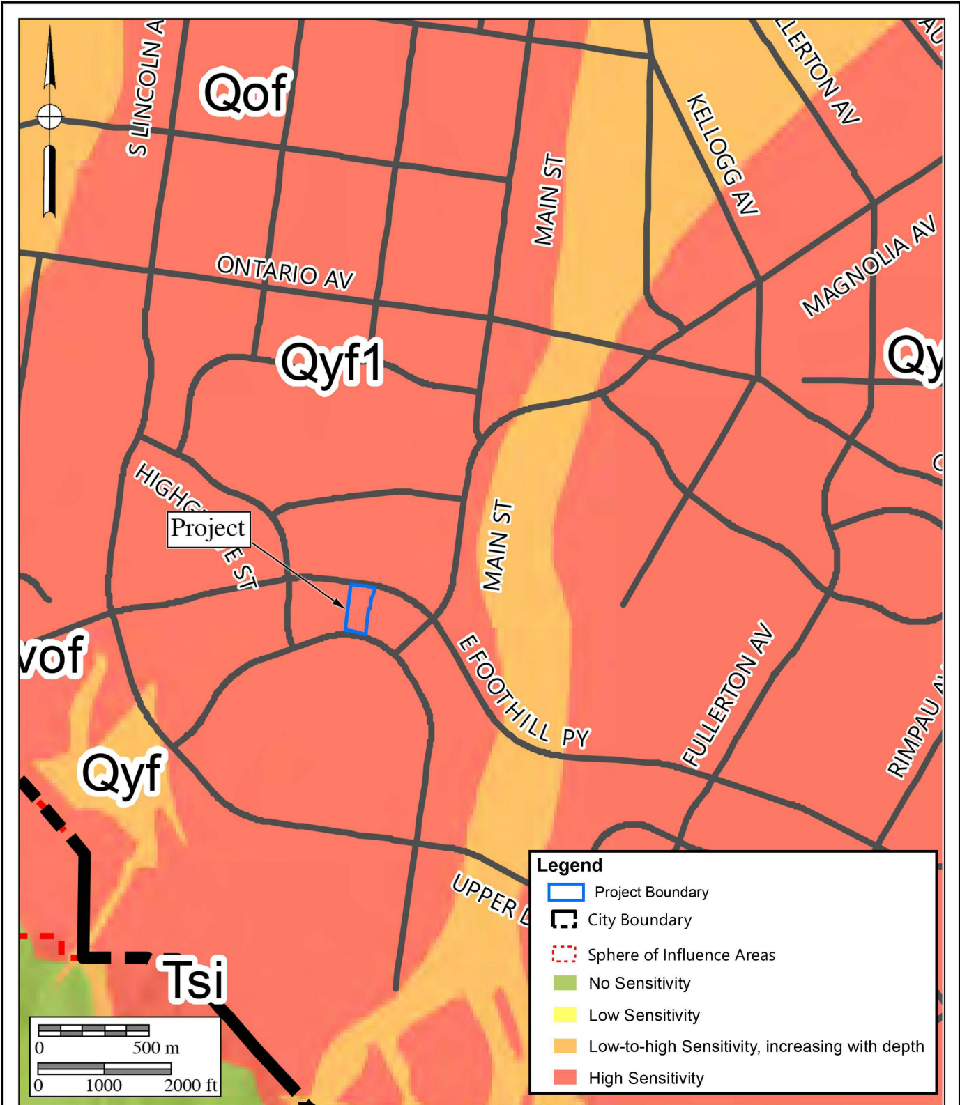
Figure 4 Paleontological Sensitivity Map The Ivy at Mountain Gate Project After City of Corona (2019)
