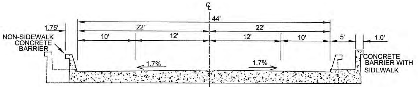
COLLECTOR STREET BRIDGE
