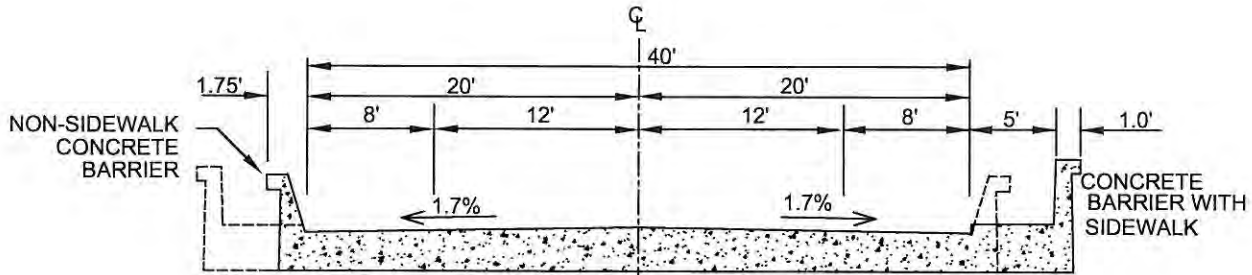
LOCAL STREET BRIDGE
