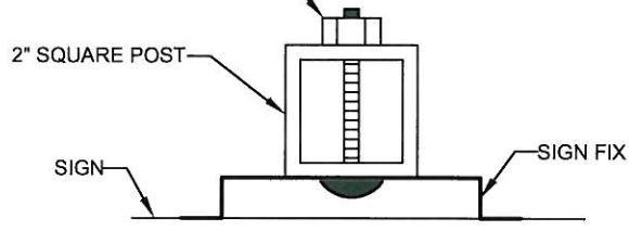
MOUNTING DETAIL PLAN VIEW
