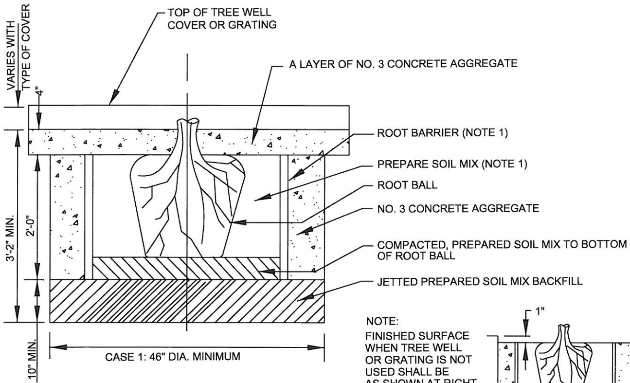
SECTION "A-A"
