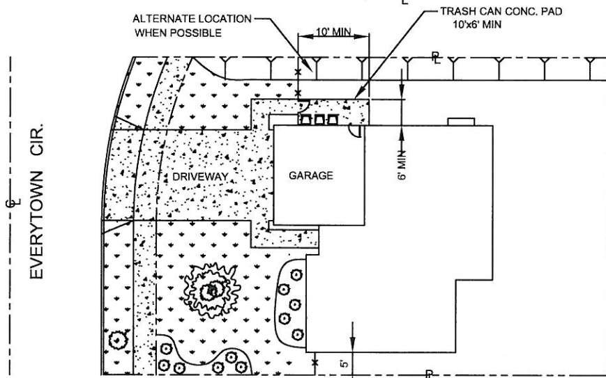
DETAIL "A" RESIDENTIAL TRASH CAN ENCLOSURE PLACEMENT
