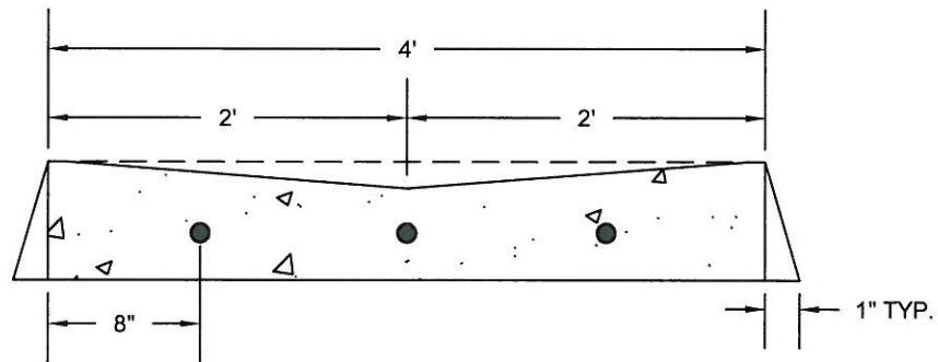
DOWEL LOCATION DETAIL
