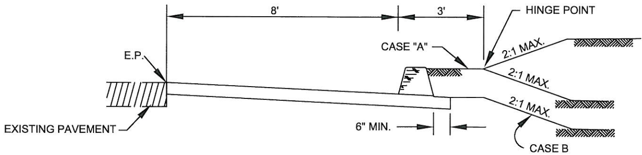
PAVED SHOULDER WITH AC BERM
