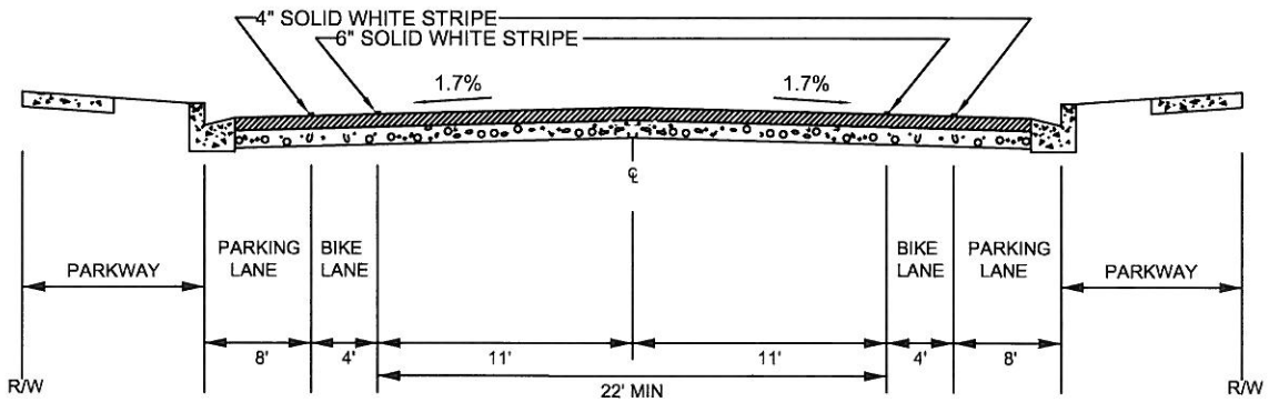
CLASS II WITH ON-STREET PARKING
