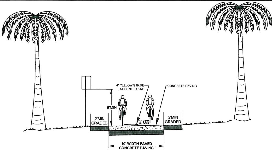
CLASS I BIKE PATH
