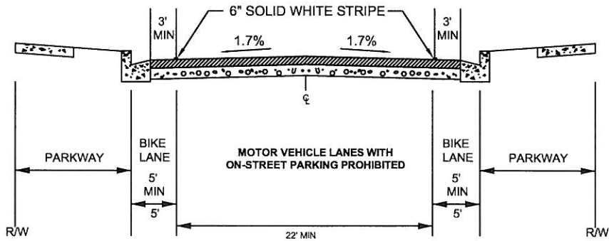
CLASS II WITHOUT ON-STREET PARKING
